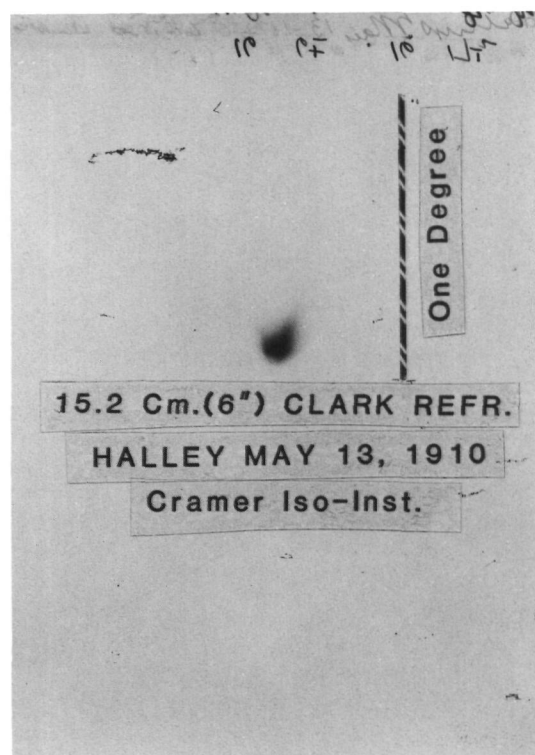
Figure 2. Photograph of Comet Halley obtained on May 13, 1910.
